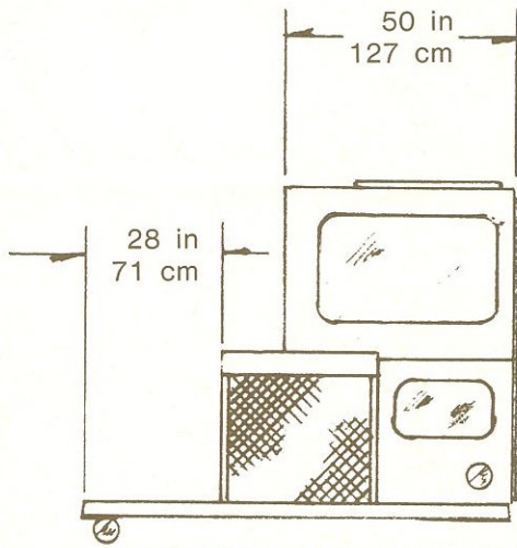
OPTIONAL ONE-MAN CAB AND SIDE DECK
